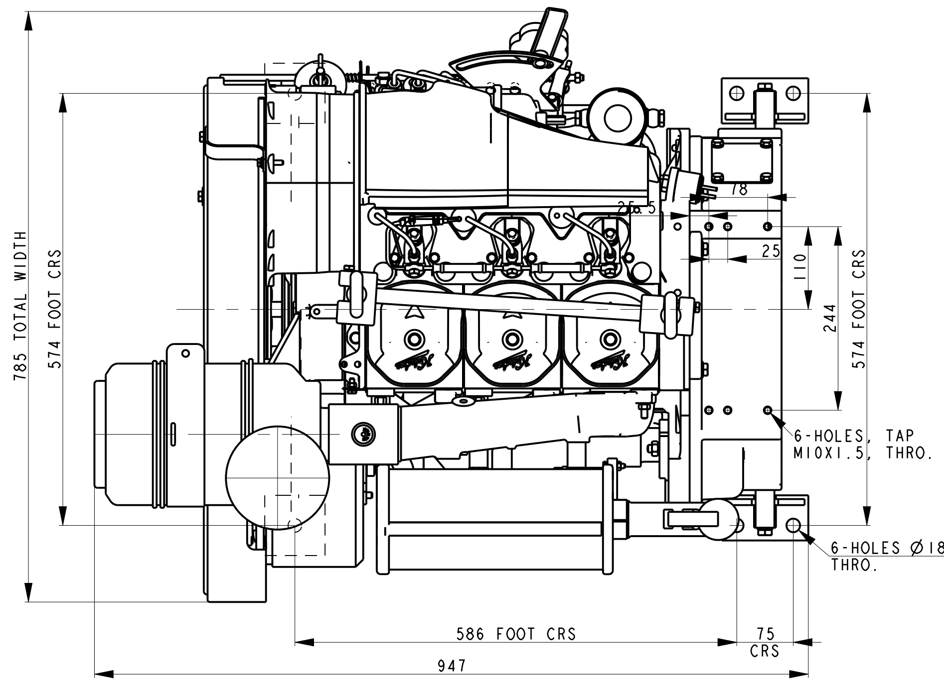
VIEW FROM TOP END
