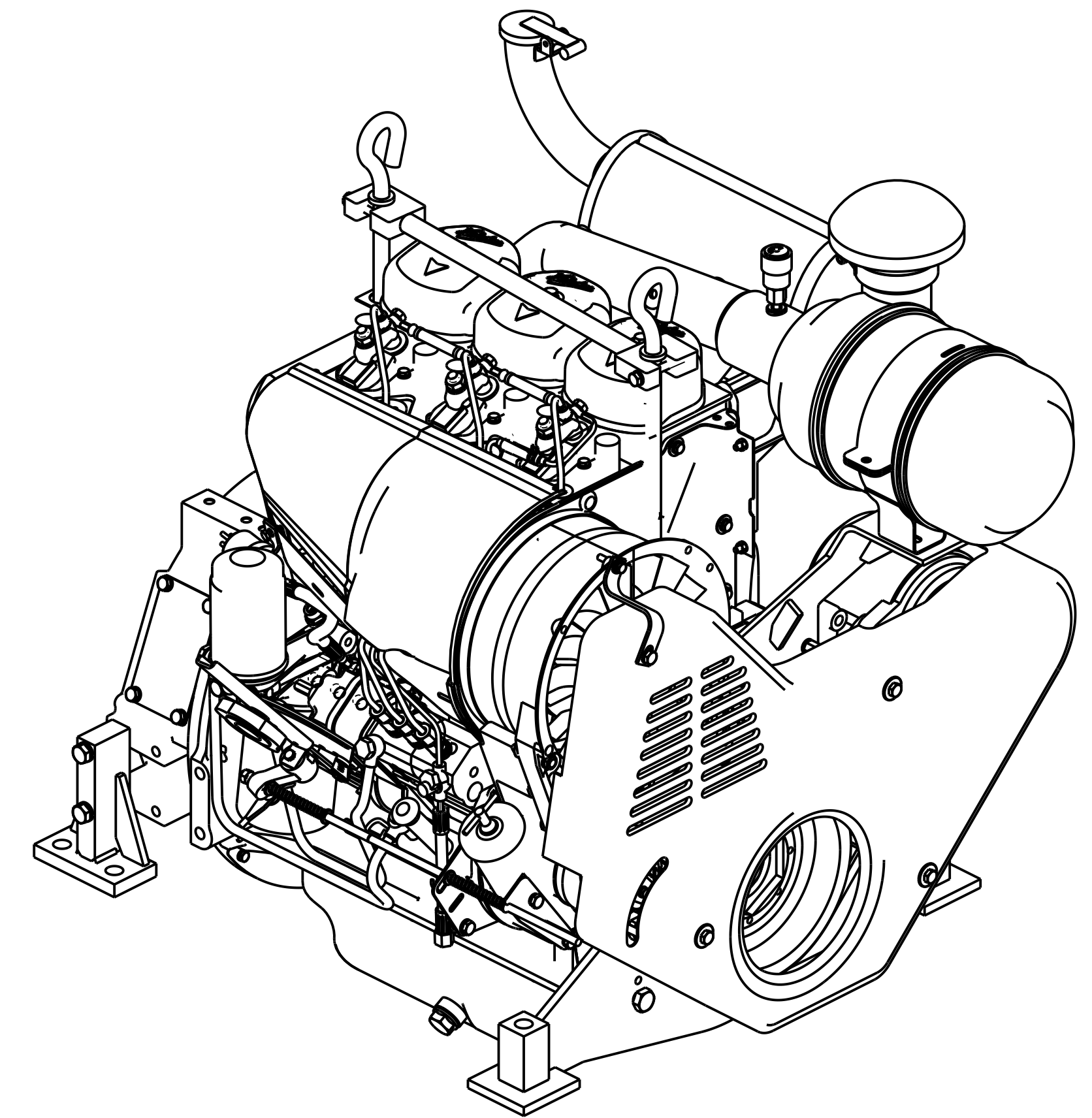
VIEW FROM FLYWHEEL END
