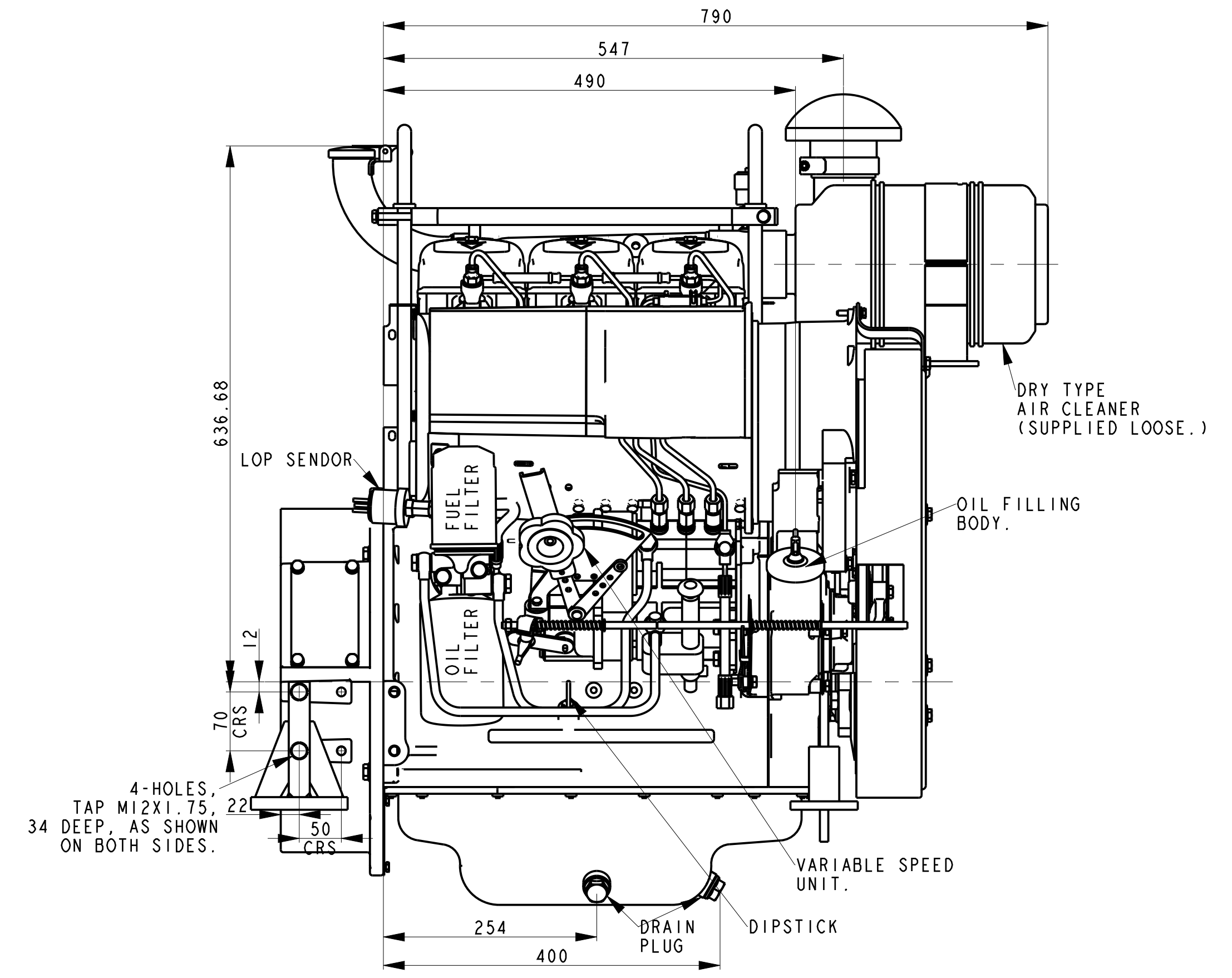
VIEW FROM FLYWHEEL END
