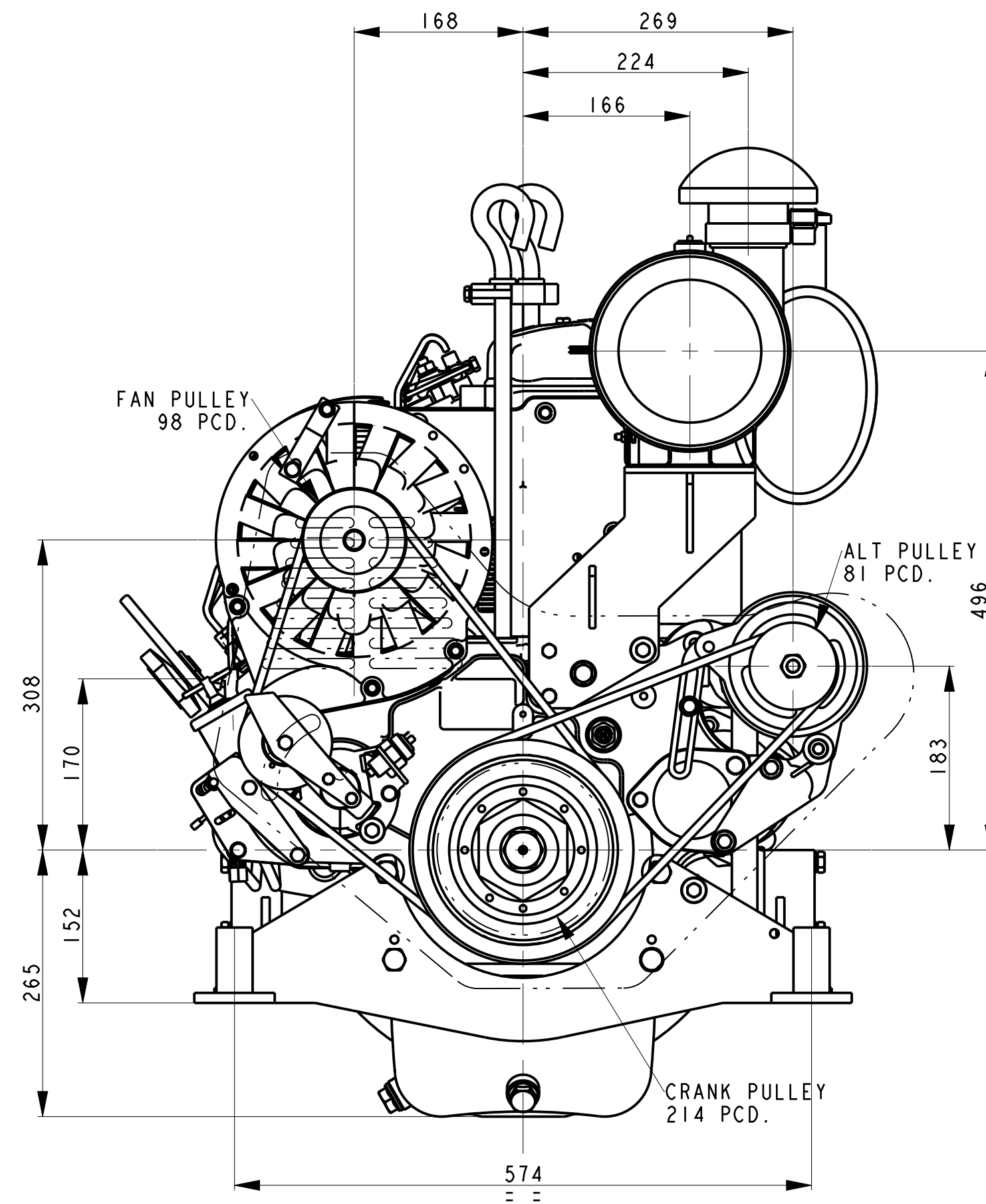
VIEW FROM GEAR END
