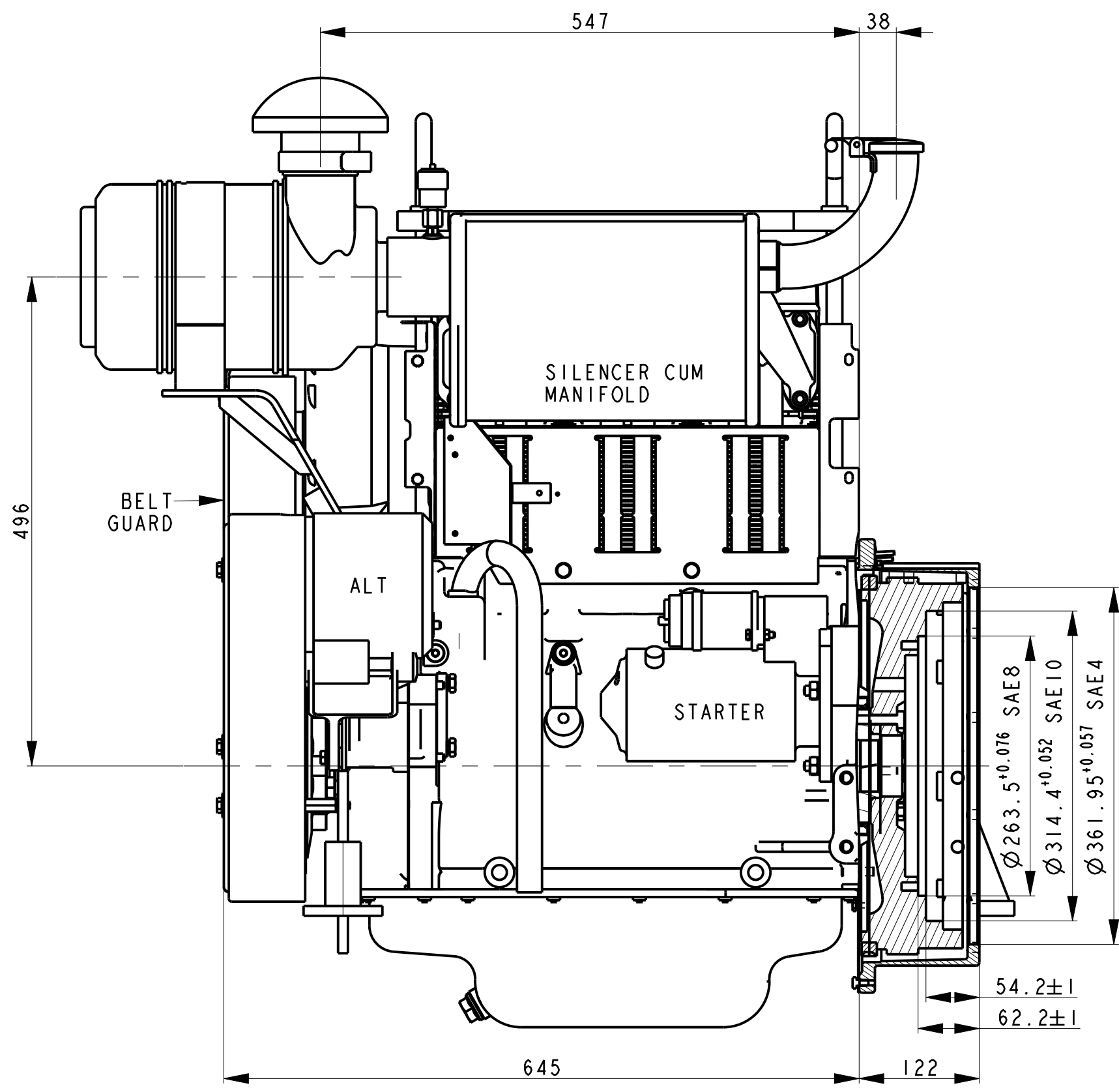
VIEW FROM STARTER END
