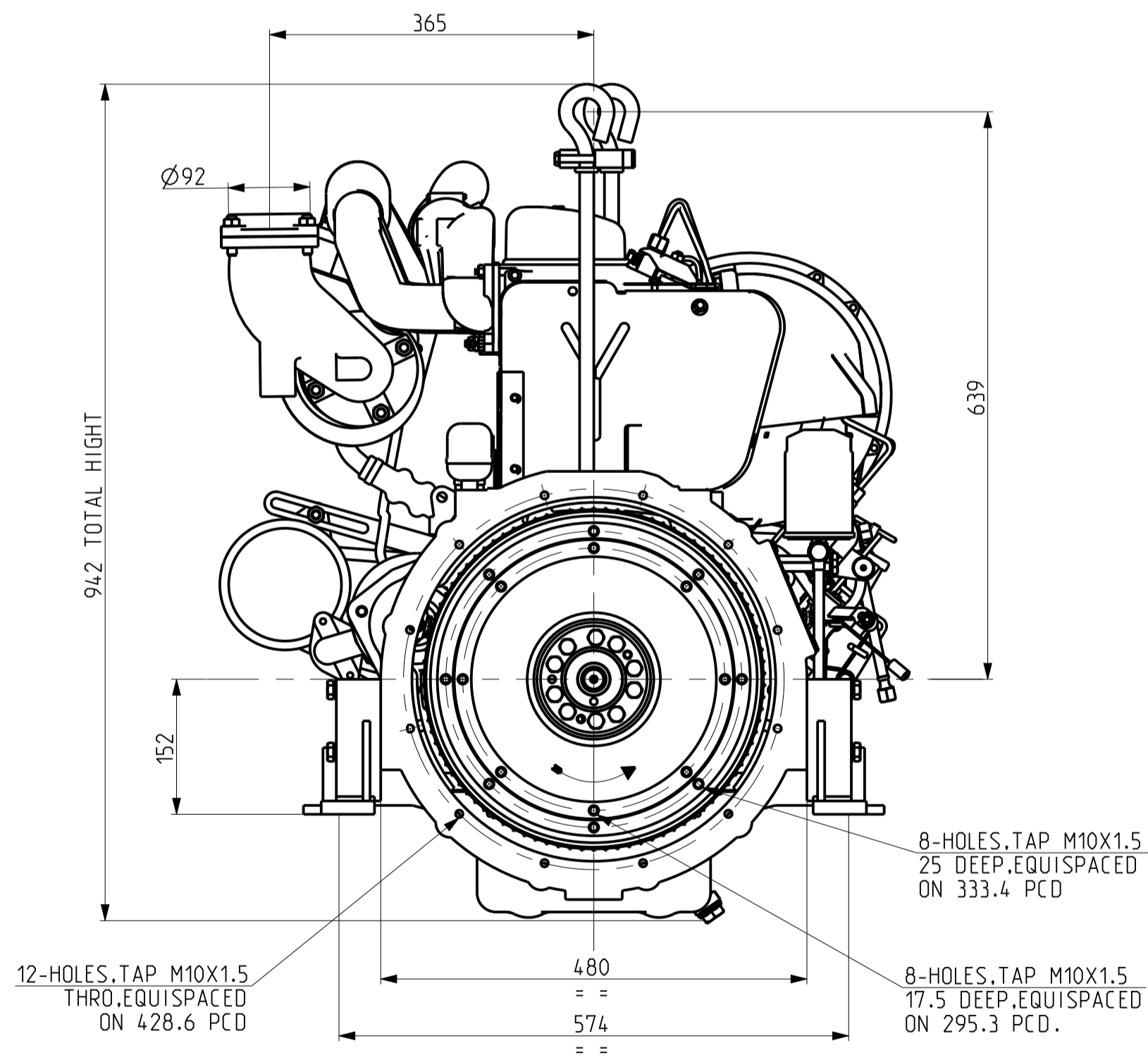
VIEW FROM FLYWHEEL END
