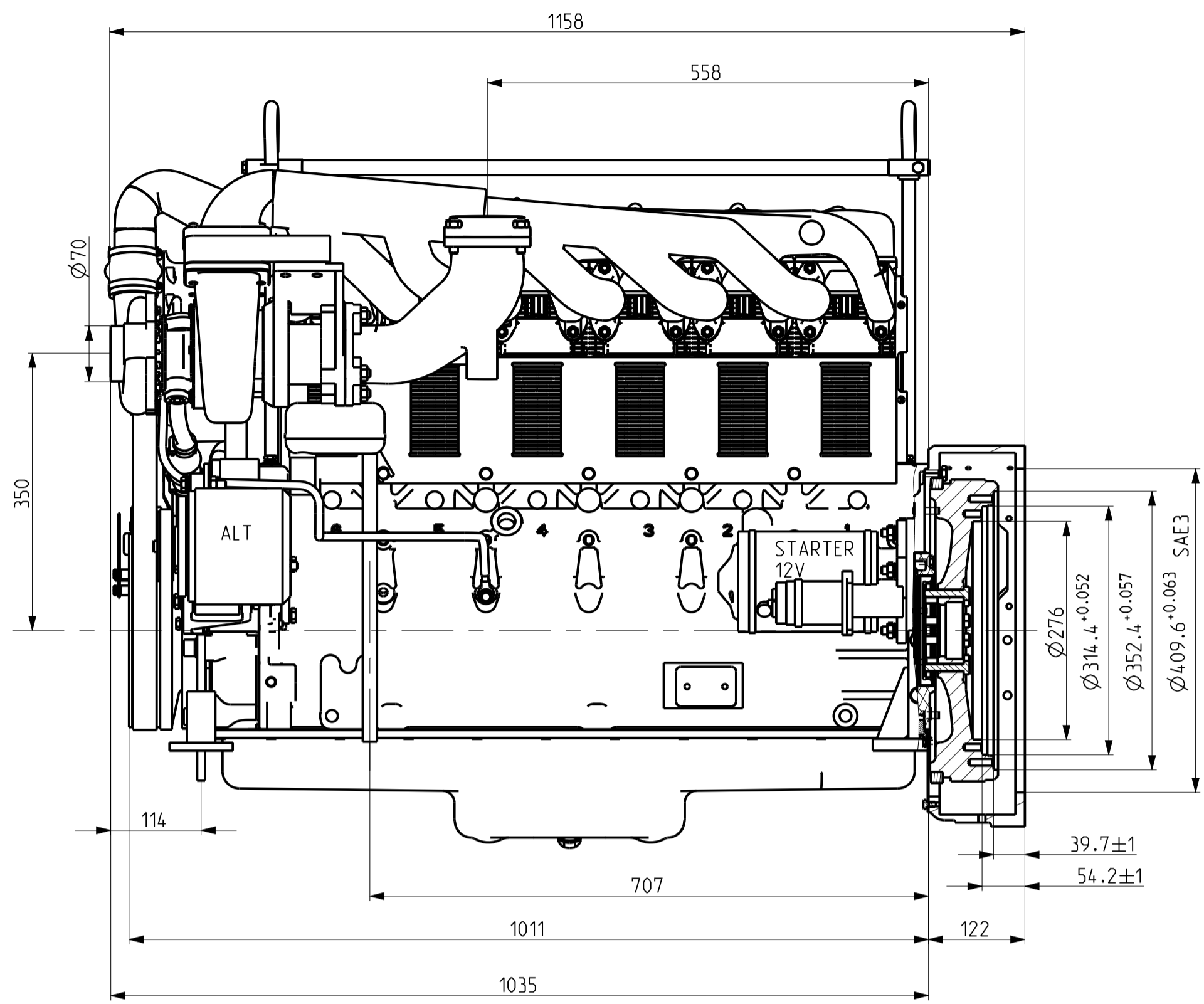
VIEW FROM STARTER END
