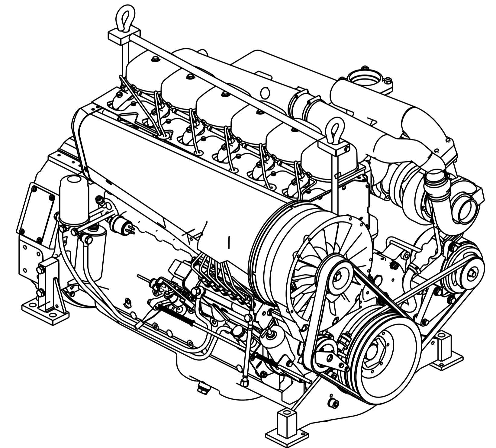
VIEW FROM F.I.P. END
