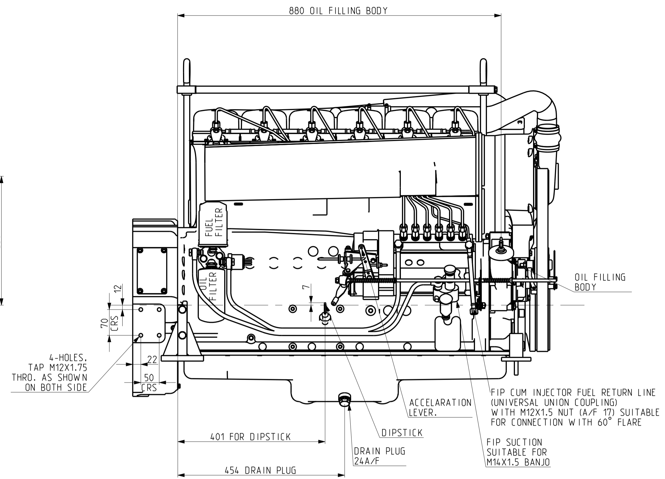
VIEW FROM F.I.P. END
