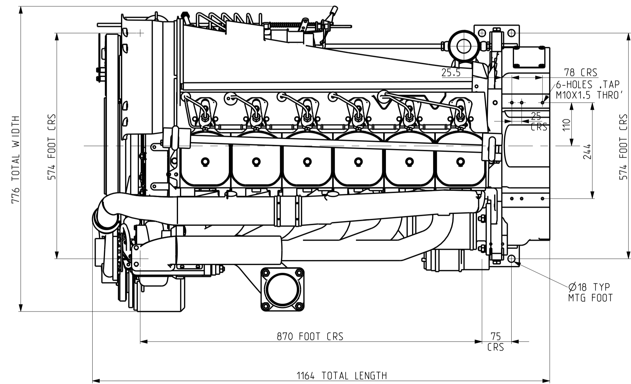
VIEW FROM TOP END
