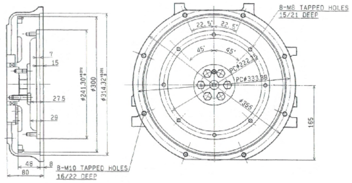
Semi SAE5/7.5" Housing & Flywheel
